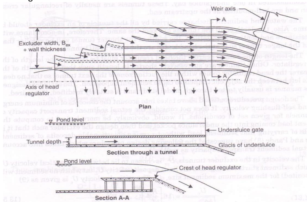
Fig: Typical Layout a Sediment Excluder
